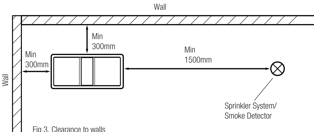
Fig 3. Clearance to walls
