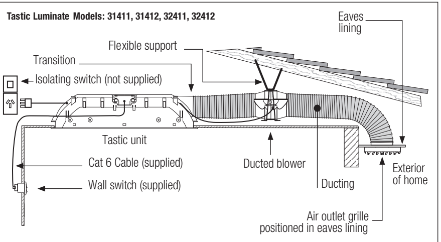
Layout of Tastic Luminate Single and Dual.
