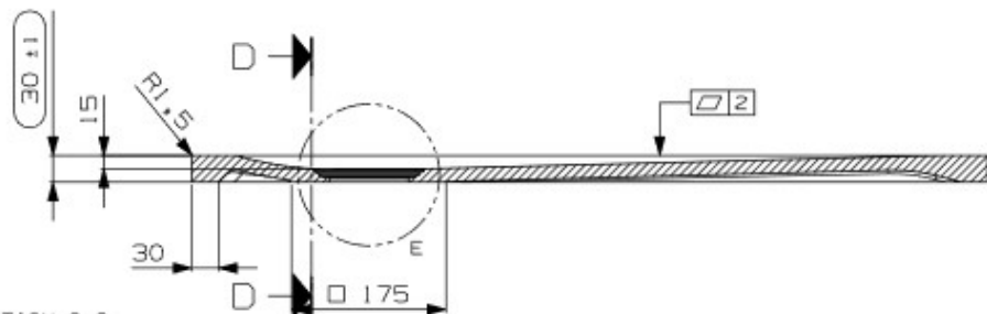
SECTION C-C SCALE 0.143:1.0
