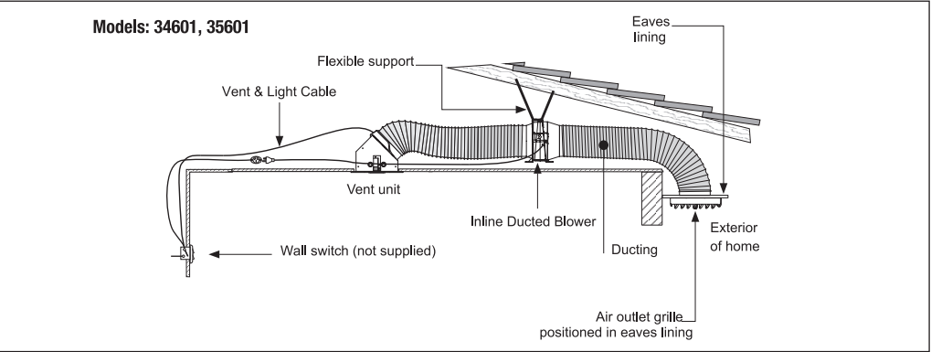
Fig. 4: Layout of Luminate Vent & Light
