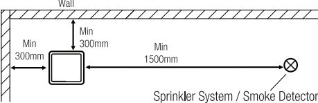
Fig. 3: Clearance to walls
