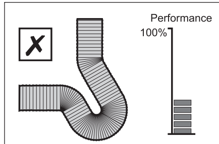
Fig. 18: Tightly compressed bends
