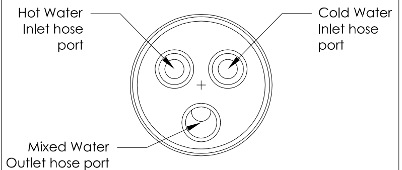
Mixer Flexi Hose Configuration Bottom View
