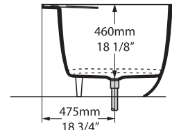
Section BB Shown with K12 Waste Kit
