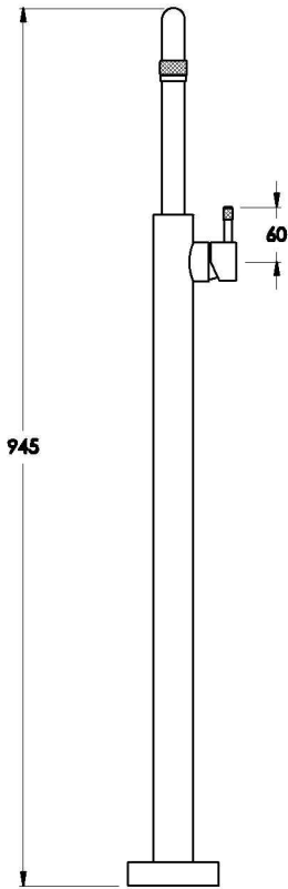
Front view
